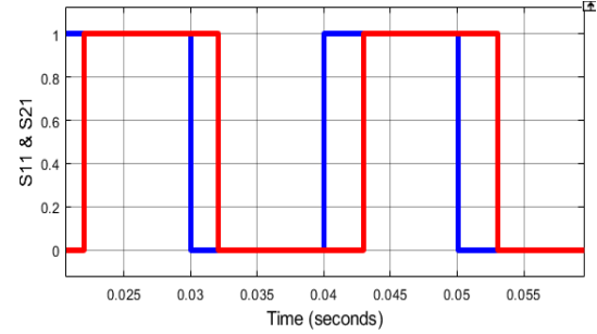
Fig 13. Simulation and test results of Phases hifted1 between port1 and port2.
