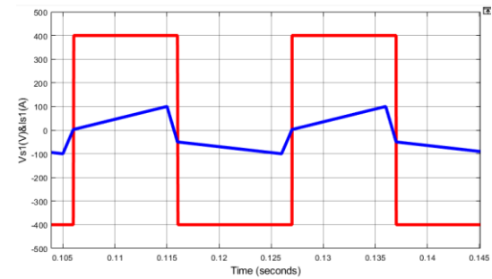
Fig 13. Simulation and test results of Phases hifted1 between port1 and port2.
