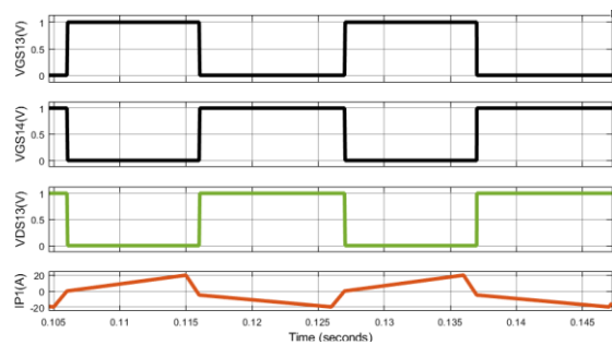
Fig 4. Simulated results of switching pulses for S13, S14 and switch voltage VDS13, current ip1.
